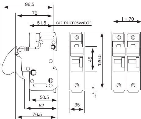
S85B9 FUSE-HOLDER-DC58x2 125A 690V For FU1, FV1 fuses (22x58 mm cylindrical)
